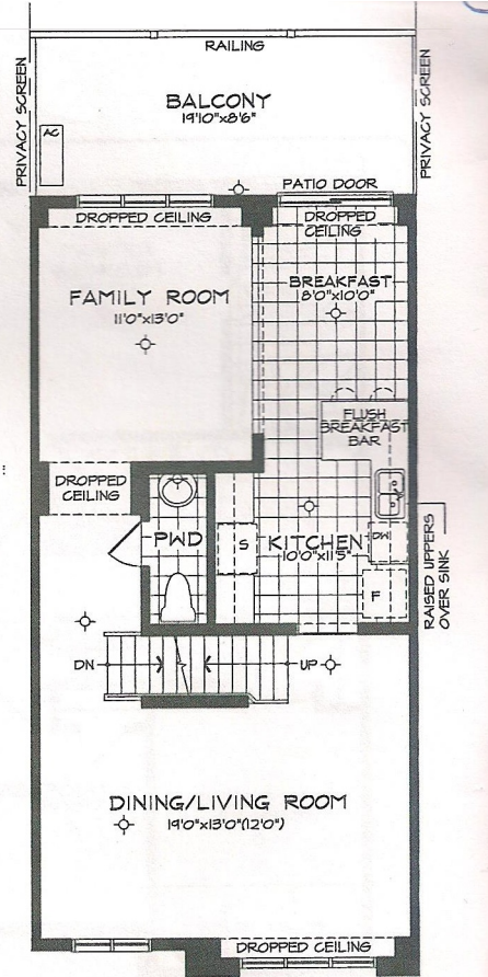
SECOND FLOOR PLAN 'B'
