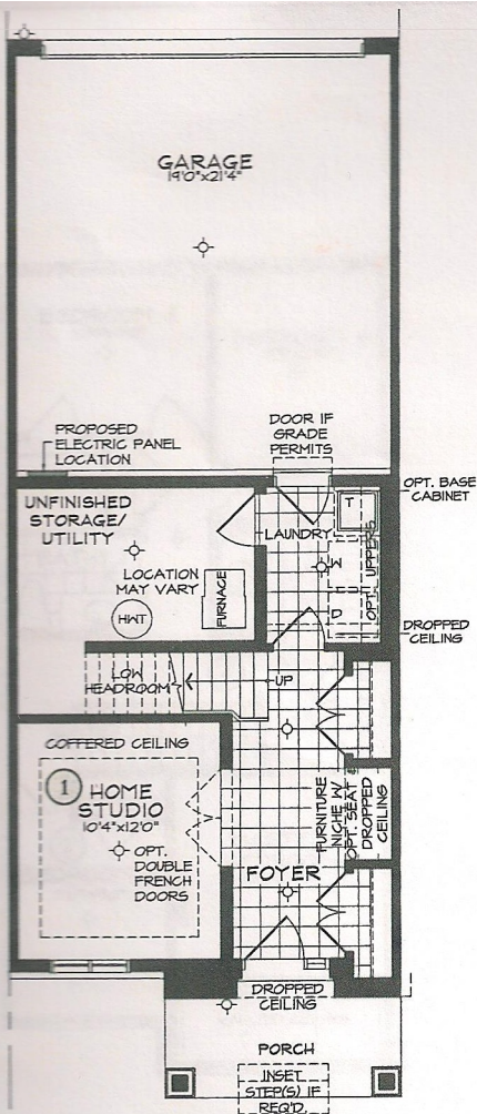
GROUND FLOOR PLAN 'B'
